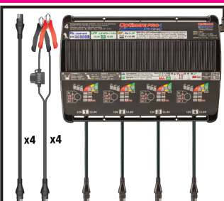
OptiMate PRO-4 DUO x4 BANK for all powersport batteries, including Pb (STD, AGM & GEL) and Li (LFP).
